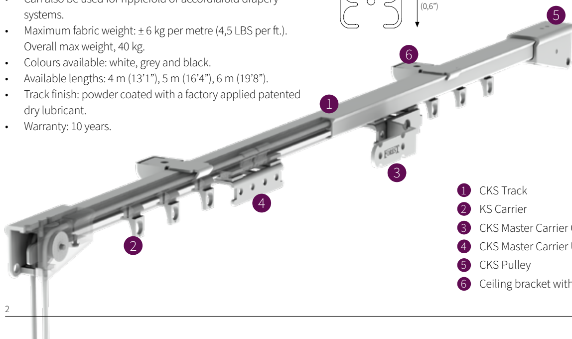
Easy installation click - position - tighten
